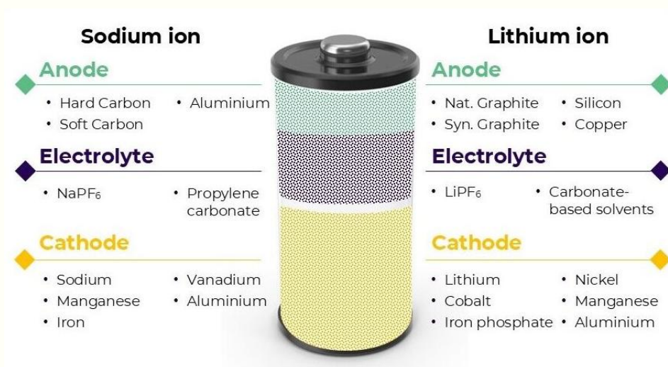
Figure 9: Sodium ion vs. Lithium-ion batteries components.
