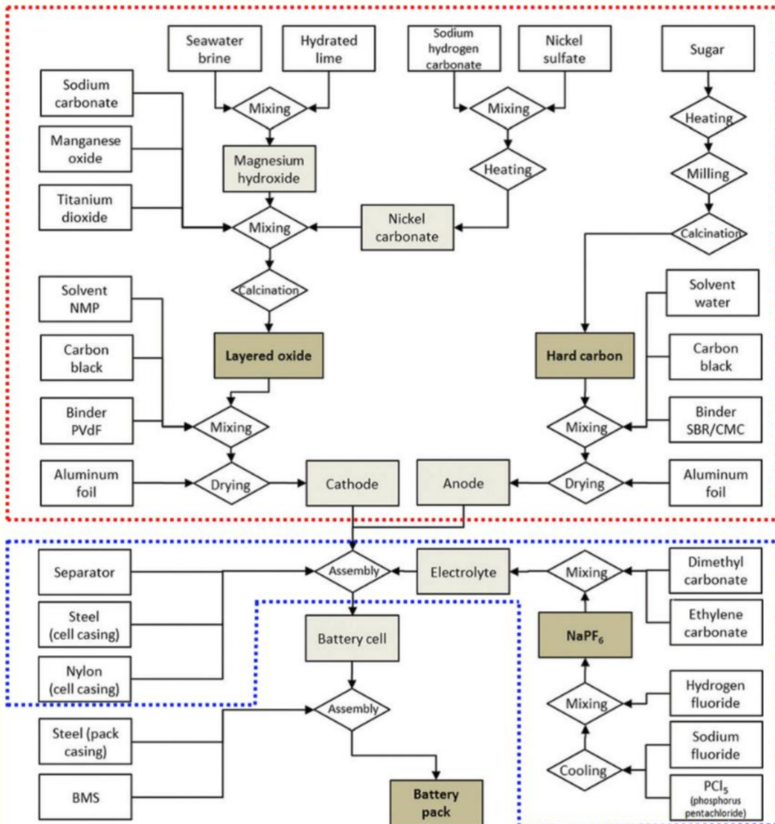
Figure 10: Comprehensive Sodium-Ion Battery Manufacturing Flowchart
